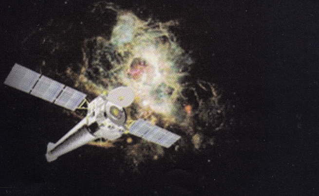
Observatorio de rayos x de la NASA Chandra space.mit.edu/.../Chandra_schematics .
